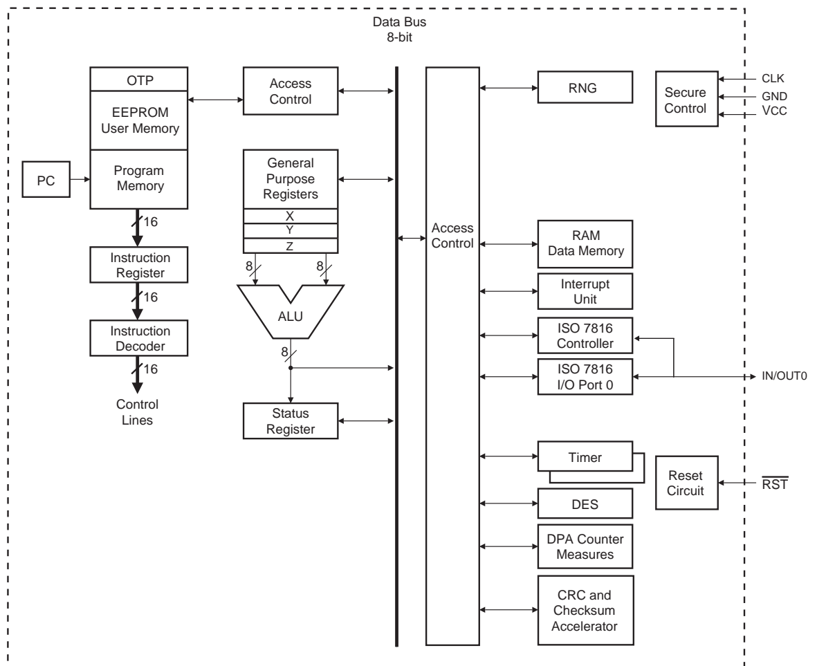
Figure 1. AT90SC9636R secureAVR Enhanced RISC Architecture
